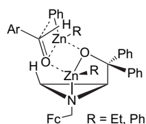
Figure 1. A possible transition state of the phenylation of arylaldehydes.
